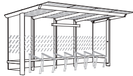
X1-V410-SS 5580 × 2500 × 2605
