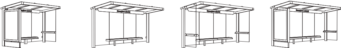
X2-330-SS+CLV 4240 × 1875 × 2735 X2-400-SS 5580 × 1875 × 2735 X2-410-SS 5580 × 1875 × 2735 X2-430-SS+CLV 5610 × 1875 × 2735
