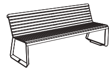
I2-301 1870 × 682 × 812
