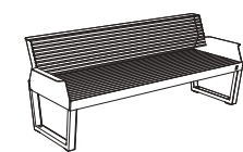
A1-361 1980 × 719 × 788
