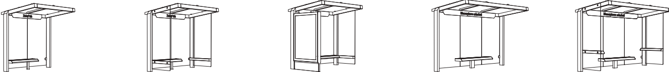
X2-200L-SS 2840 × 1875 × 2735 X2-210L-SS 2840 × 1875 × 2735 X2-230R-SS+CLV 2870 × 1875 × 2735 X2-300-SS 4210 × 1875 × 2735 X2-310-SS 4210 × 1875 × 2735
