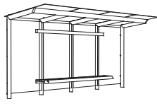
X1-400-SS 5545 × 1738 × 2605
