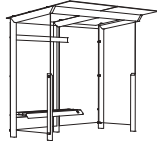
X1-210L-SS 2800 × 1738 × 2605
