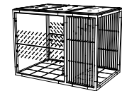
Y3-SET2102 3250 × 2165 × 2450
